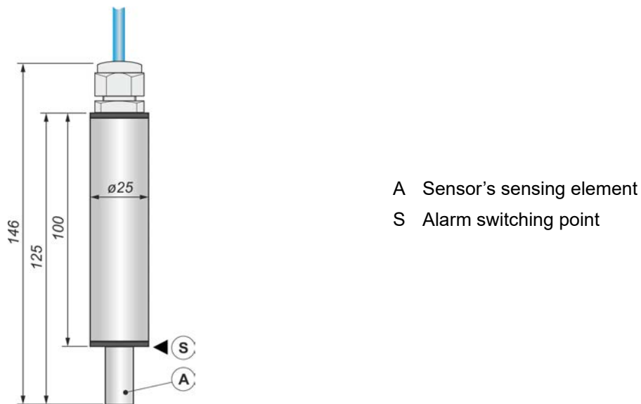
Figure 1. High liquid level sensor idOil-LIQ – structure and dimensions (mm)
