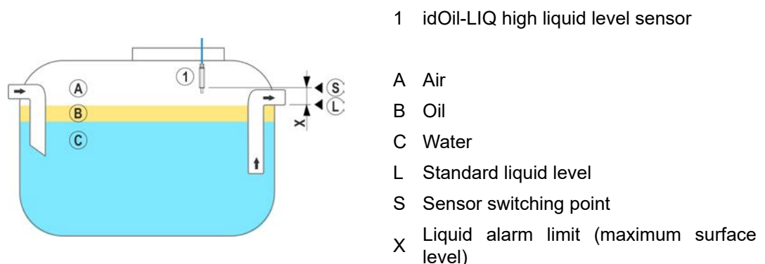
Figure 4. Installing the idOil-LIQ high liquid limit sensor
